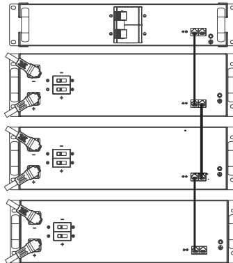
Figure 12. Grounding the Battery Module Combiner
